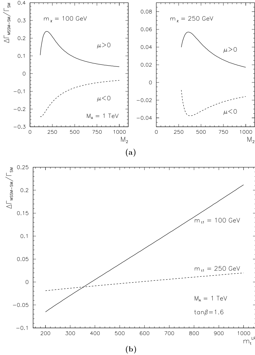
Fig. 7. The deviation of the h \rightarrow Z\gamma decay width from the Standard Model value [in %] for \tan\beta = 1.6 and the loop masses m_i = 100 and 250 GeV. a Deviations due to the chargino loops as a function of M_2 for both signs of \mu , and b deviations due to the top squark loops as a function of m_t^{LR}
