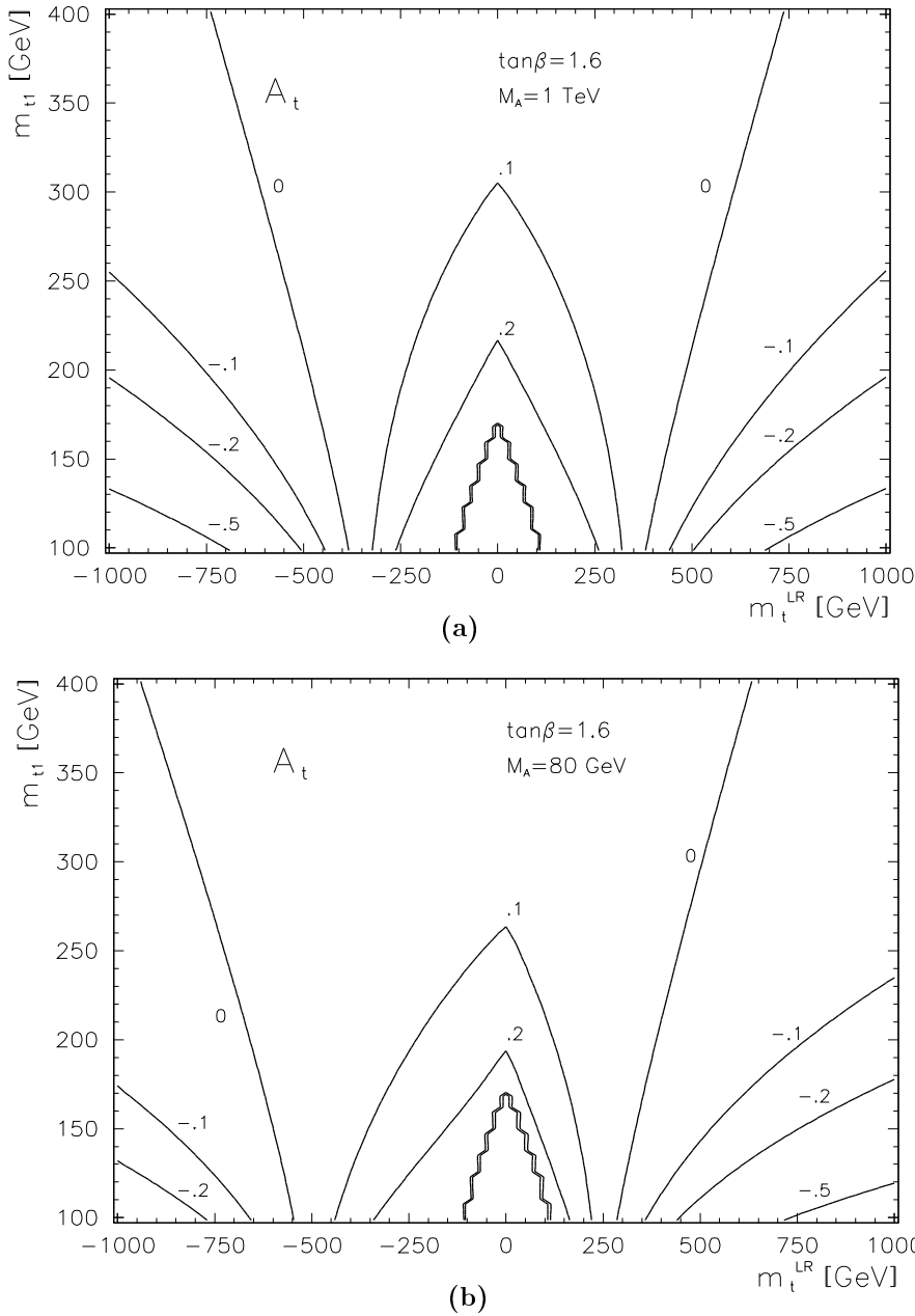
Fig. 5. Contours in the (m_t^{LR}, m_{\tilde{t}_1}) plane, for which the contribution of the top squark loops to the hZ\gamma coupling is |A_{\tilde{t}}| = 0.5, 0.2 and 0.1 for M_A = 1 TeV a and M_A = 80 GeV b with \tan\beta = 1.6
