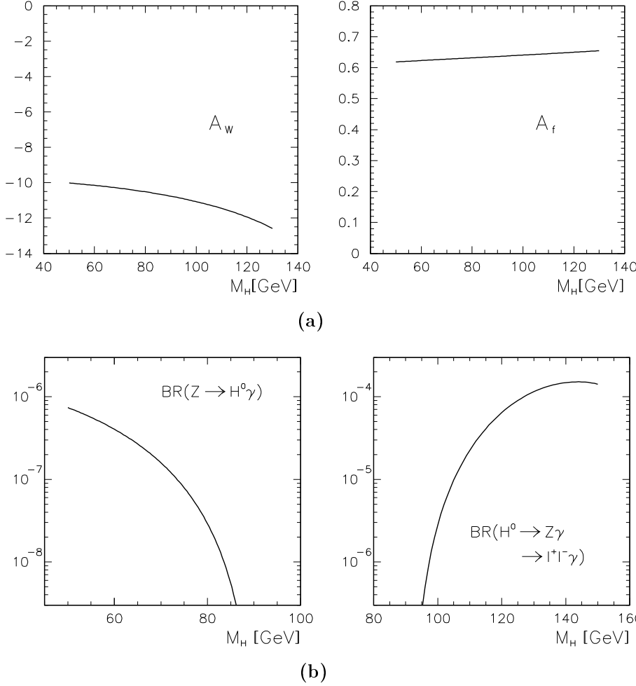
Fig. 2. The W and top quark form factors in the SM as a function of the Higgs boson mass a and the branching ratios of the decays H^0 \rightarrow Z\gamma \rightarrow l^+l^-\gamma and Z \rightarrow H^0\gamma in the SM b
